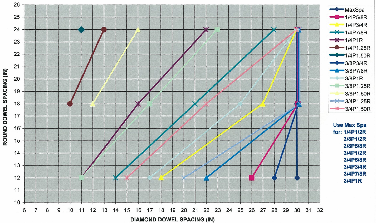
DIAMOND DOWEL VS. ROUND DOWEL SPACING
